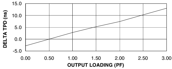
22LV10CZ/CQZ DELTA T_{PD} VS. OUTPUT LOADING
